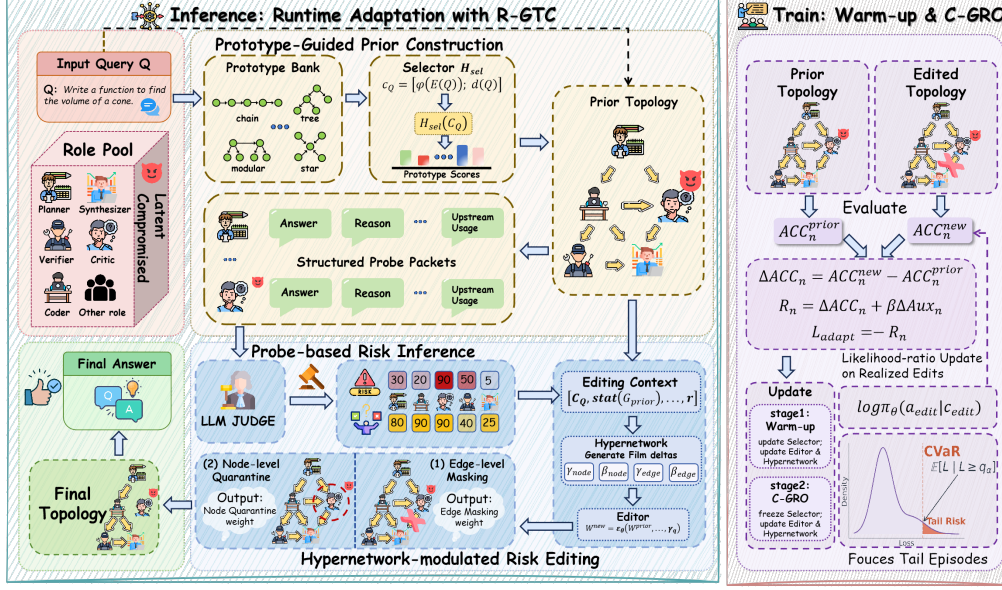
Figure 2: Architecture illustration of RIGOR. (a) The left part shows the inference phase that first probes agent behavior given a query, then uses an LLM judge to estimate per-agent risk and uncertainty, and finally applies node quarantine and edge masking for robust topology. (b) The right part shows the training phase that first warms up core modules, then optimizes high-loss tail episodes via CVaR, and finally updates the topology editor. Please refer to Appendix I.1 and I.2 for case study.
