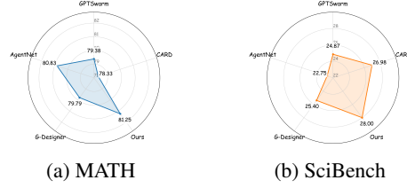
Figure 5: Clean-setting comparison . RIGOR attains higher accuracy than the compared adaptive-topology MAS methods when no agent is compromised, using GPT-4o-mini as the backbone.
