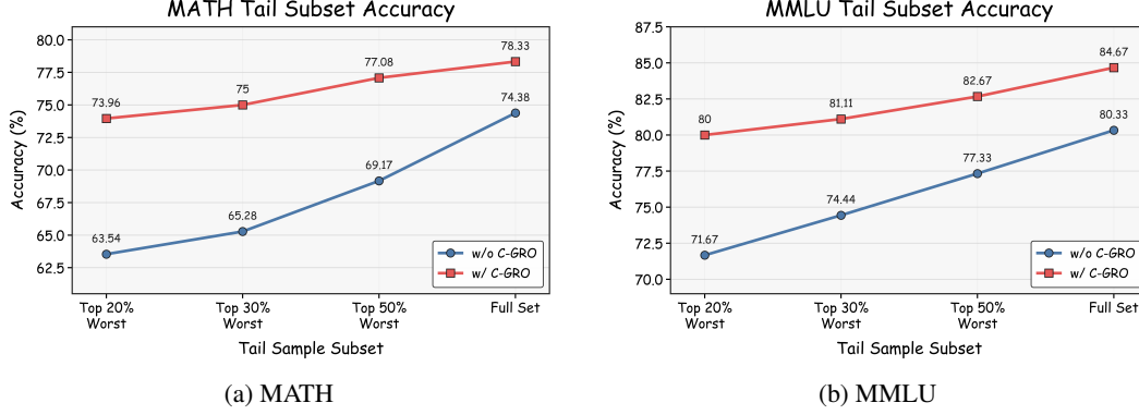
Figure 6: Tail-subset stability of C-GRO. We compare variants without and with C-GRO on progressively larger worst-sample subsets. C-GRO consistently improves the high-loss tail and keeps the curve higher as the subset expands from the worst 20% to the full set.
