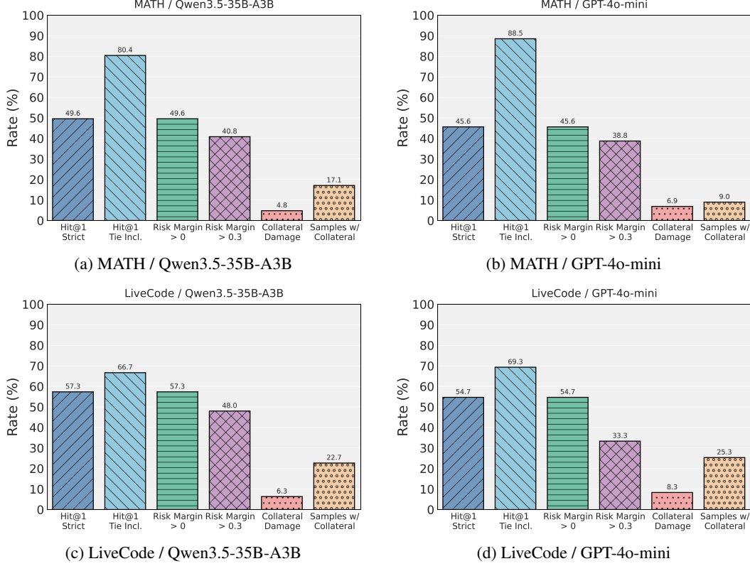
Figure 9: LLM-judge diagnostics on MATH and LiveCode under two backbone models. Hit@1 strict measures whether the single highest-risk agent is the compromised agent, while tie-inclusive Hit@1 also counts cases where the compromised agent is tied for the maximum risk score. The remaining bars report positive risk-margin rates and collateral-risk indicators.
