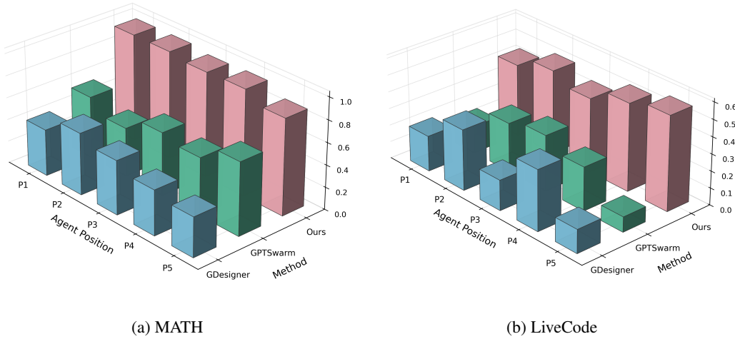
Figure 8: Robustness to compromised-agent position. For each dataset, we aggregate the query-varying main-table runs by the realized compromised-agent position and report the resulting score for each method using Qwen3.5-35B-A3B. RIGOR remains consistently stronger across positions, indicating that its robustness is not driven by a favorable distribution of attack locations.
