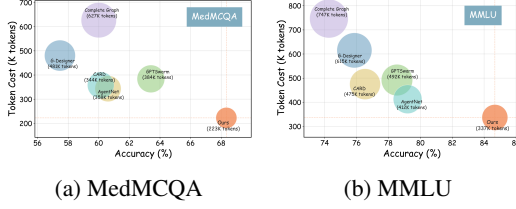
Figure 4: Accuracy-token trade-off . RIGOR reaches a favorable accuracy-token trade-off compared with baseline MAS methods on MedMCQA and MMLU; token cost counts prompt-plus-completion tokens from the executed pipeline, including diagnostic probe/judge calls when invoked.
