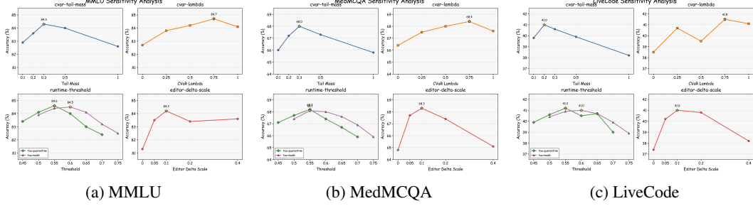
Figure 7: Sensitivity analysis on MMLU, MedMCQA, and LiveCode. Across datasets, the best region appears at a moderate CVaR tail mass, a nonzero CVaR mixing weight, intermediate runtime editing thresholds, and a nonzero FiLM delta scale.
