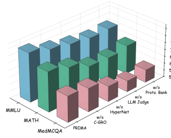
Figure 3: Component attribution in RIGOR . Removing key modules generally degrades performance.
